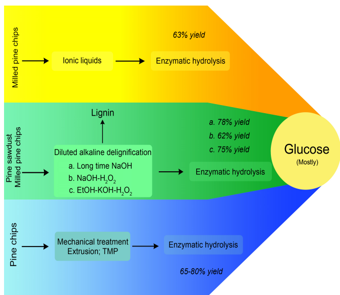
Fig.3. Schematic representation of reported pretreatments on pine producing medium enzymatic hydrolysis yields.
