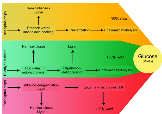
Fig.7. Schematic representation of reported pretreatments on eucalyptus producing high enzymatic hydrolysis yields.
