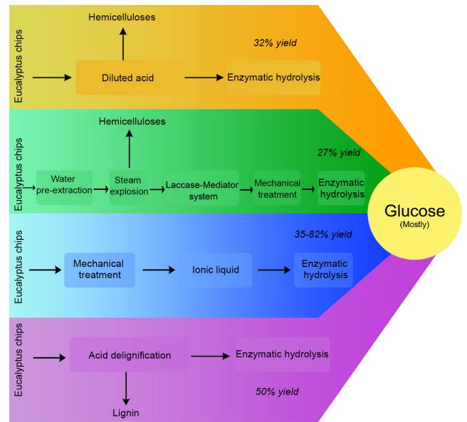
Fig.5. Schematic representation of reported pretreatments on eucalyptus producing low enzymatic hydrolysis yields.
