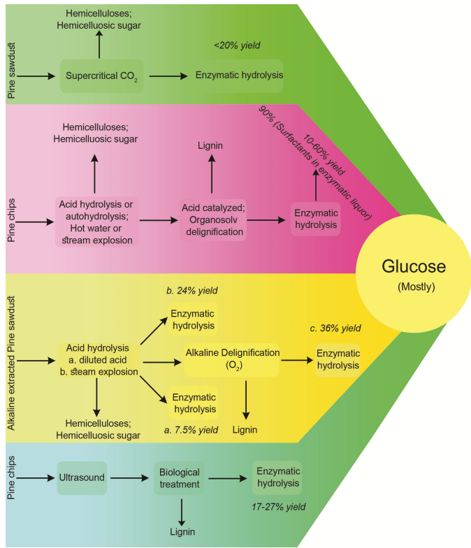
Fig.2. Schematic representation of reported pretreatments on pine producing low enzymatic hydrolysis yields.
