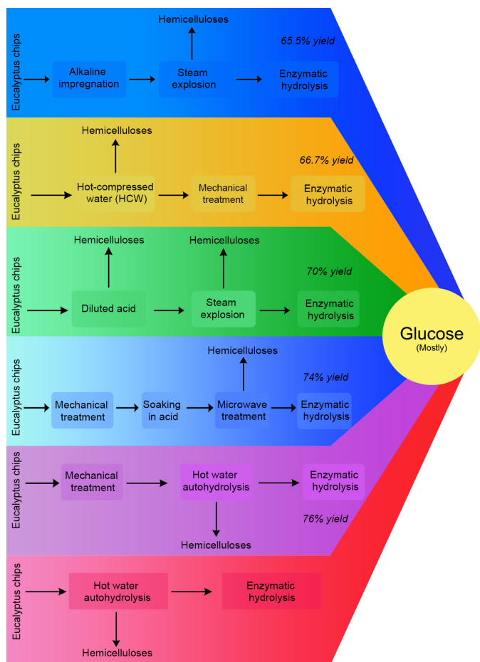
Fig.6. Schematic representation of reported pretreatments on eucalyptus producing medium enzymatic hydrolysis yields.
